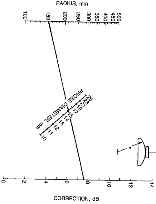
FIGURE D1. COMPENSATION FOR CURVATURE
