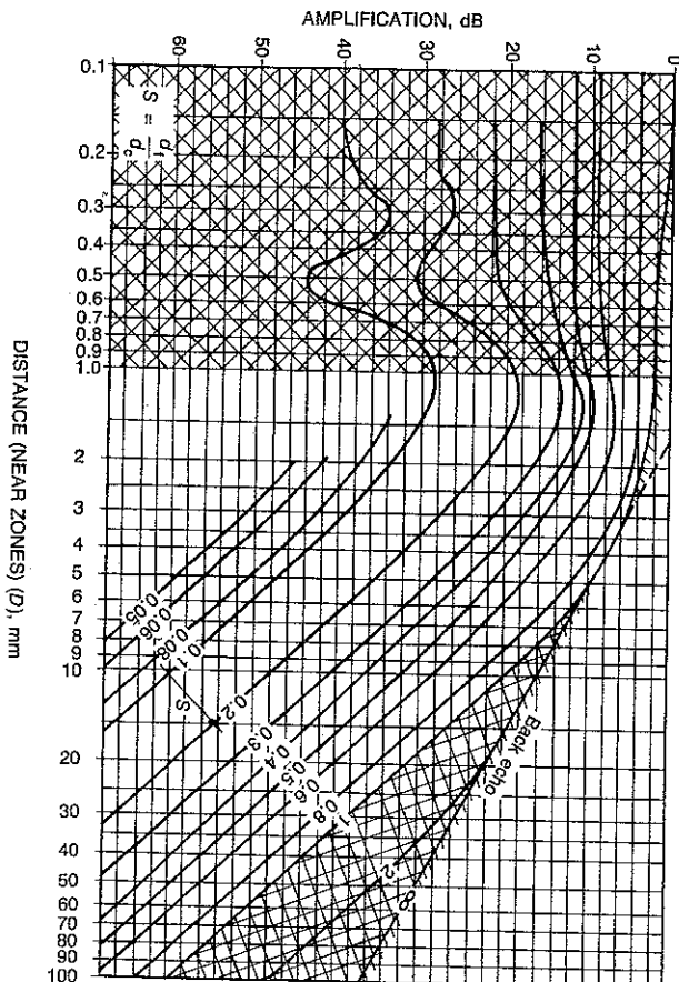
FIGURE C1. REFLECTIVITY DIAGRAM FOR NORMAL PROBES
