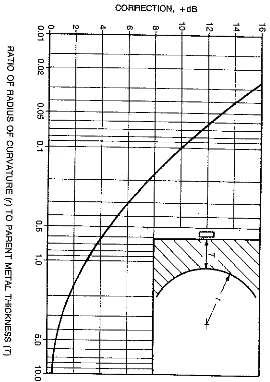
FIGURE D2. CORRECTIONS FOR VARIOUS VALUES OF r/T
